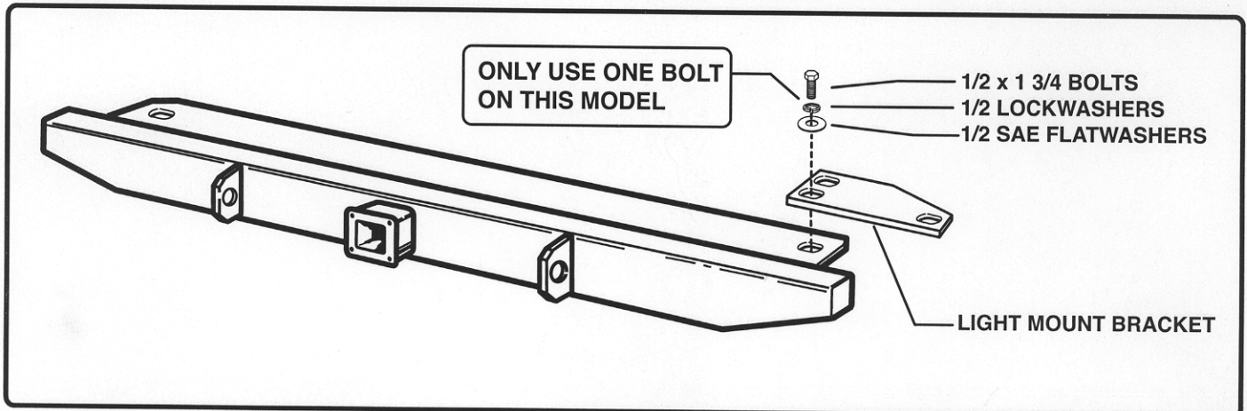
76-95 CJ-7 & JEEP WRANGLER (YJ) INSTALLATION
